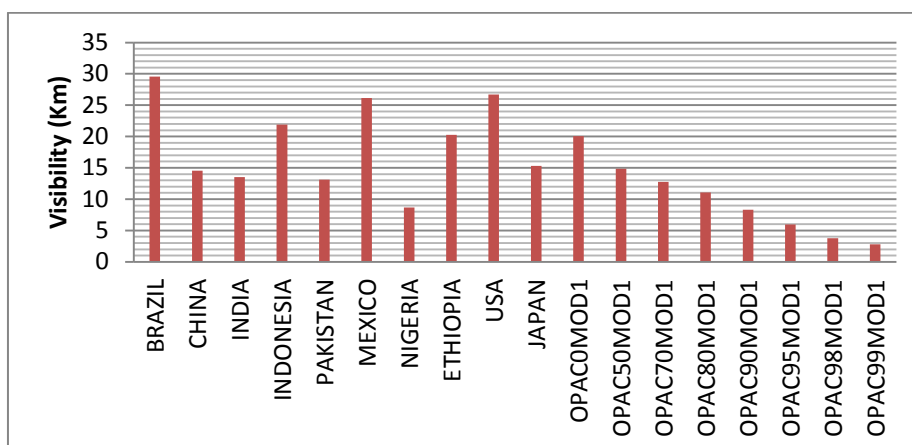
Fig 11. Histogram plot for OPAC SOOT Model 1 Visibilities and MERRA averaged visibilities for ten countries (Nigeria, Ethiopia, Brazil, USA, Pakistan, Mexico, Japan, China, Indonesia and India)
