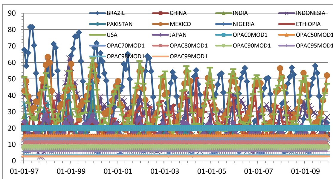
Fig 12. Visibility plot for OPAC SOOT Model 1 Visibilities and MERRA averaged visibilities for ten countries (Nigeria, Ethiopia, Brazil, USA, Pakistan, Mexico, Japan, China, Indonesia and India)
