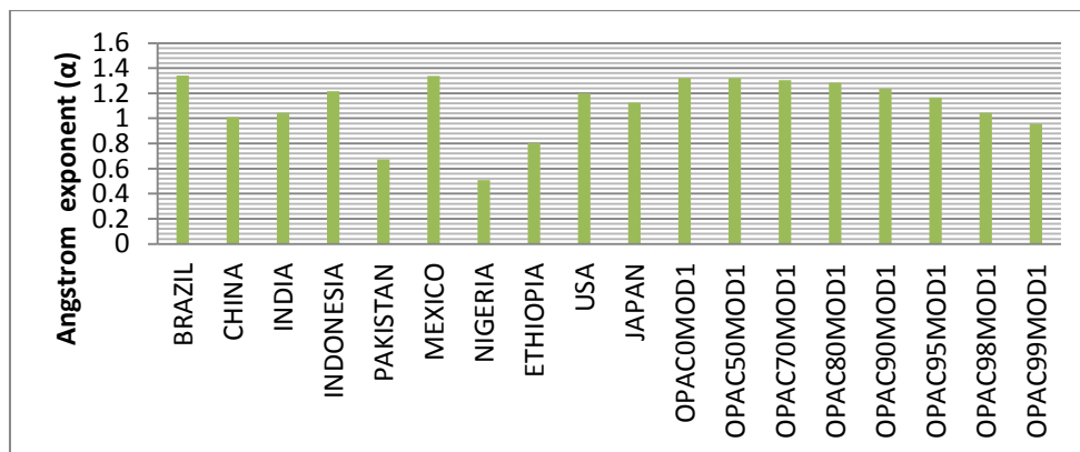
Fig 1. Histogram plot for OPAC WASO Model 1 Angstrom Exponent ( \alpha ) and MERRA averaged Angstrom Exponent ( \alpha ) for ten countries (Nigeria, Ethiopia, Brazil, USA, Pakistan, Mexico, Japan, China, Indonesia and India)
