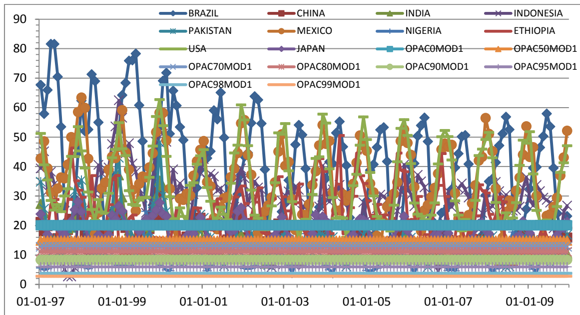
Fig 4. Visibility plot for OPAC WASO Model 1 Visibilities and MERRA averaged visibilities for ten countries (Nigeria, Ethiopia, Brazil, USA, Pakistan, Mexico, Japan, China, Indonesia and India
