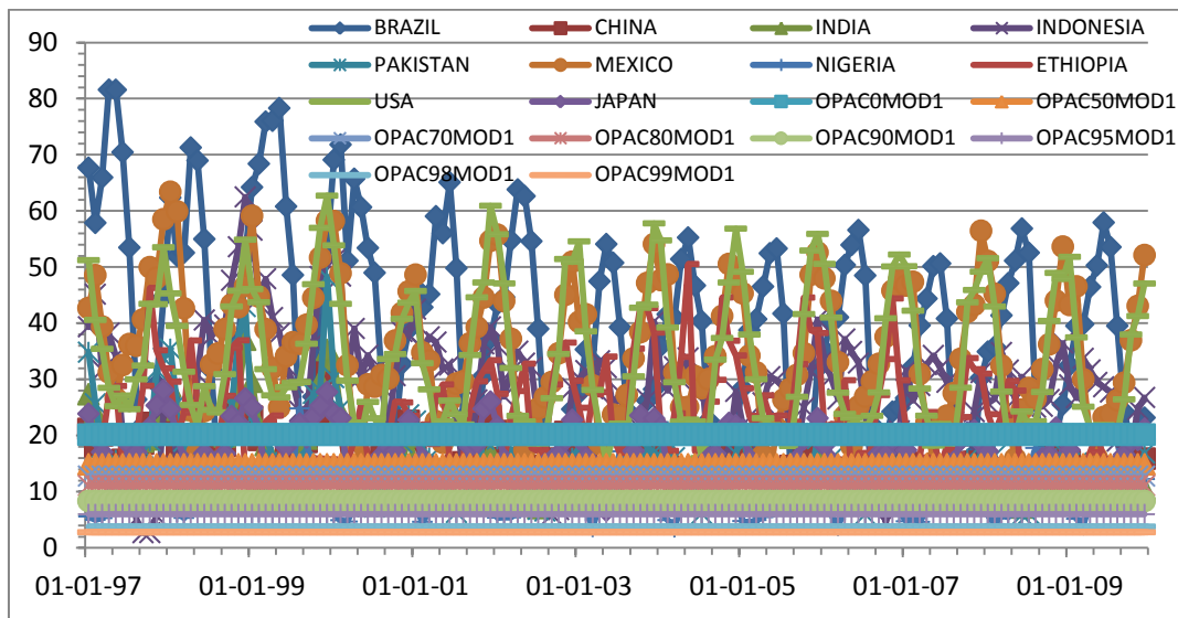
Fig 8. Visibility plot for OPAC INSO Model 1 Visibilities and MERRA averaged visibilities for ten countries (Nigeria, Ethiopia, Brazil, USA, Pakistan, Mexico, Japan, China, Indonesia and India)
