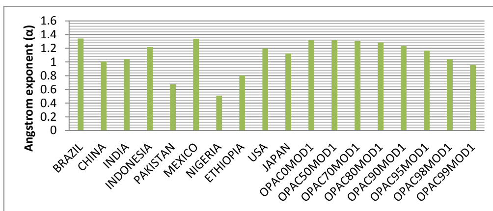
Fig 9. Histogram plot for OPAC SOOT Model 1 Angstrom Exponent ( \alpha ) and MERRA averaged Angstrom Exponent ( \alpha ) for ten countries (Nigeria, Ethiopia, Brazil, USA, Pakistan, Mexico, Japan, China, Indonesia and India)
