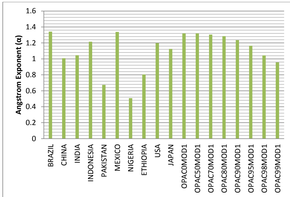
Fig. 5. Histogram plot for OPAC INSO Model 1 Angstrom Exponent ( \alpha ) and MERRA averaged Angstrom Exponent ( \alpha ) for ten countries (Nigeria, Ethiopia, Brazil, USA, Pakistan, Mexico, Japan, China, Indonesia and India)
