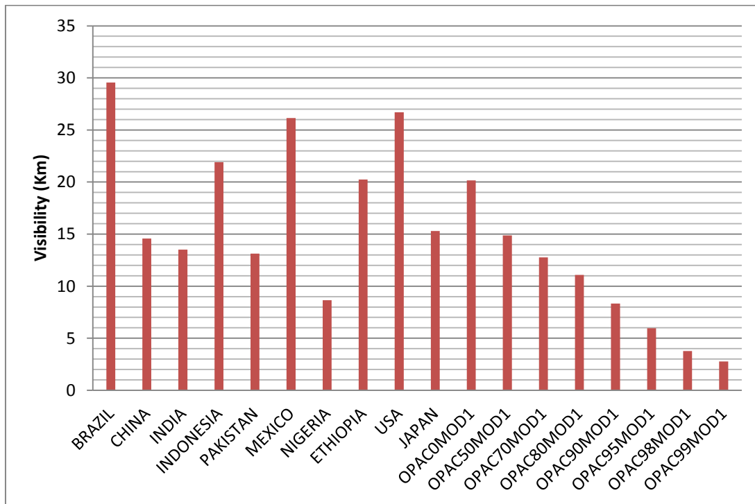
Fig. 7. Histogram plot for OPAC INSO Model 1 Visibilities and MERRA averaged visibilities for ten countries (Nigeria, Ethiopia, Brazil, USA, Pakistan, Mexico, Japan, China, Indonesia and India)
