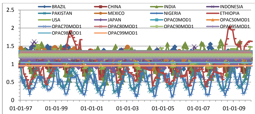
Fig. 10. Angstrom Exponent ( \alpha ) plot for OPAC SOOT Model 1 Angstrom Exponent ( \alpha ) and MERRA averaged Angstrom Exponent ( \alpha ) for ten countries (Nigeria, Ethiopia, Brazil, USA, Pakistan, Mexico, Japan, China, Indonesia and India)
