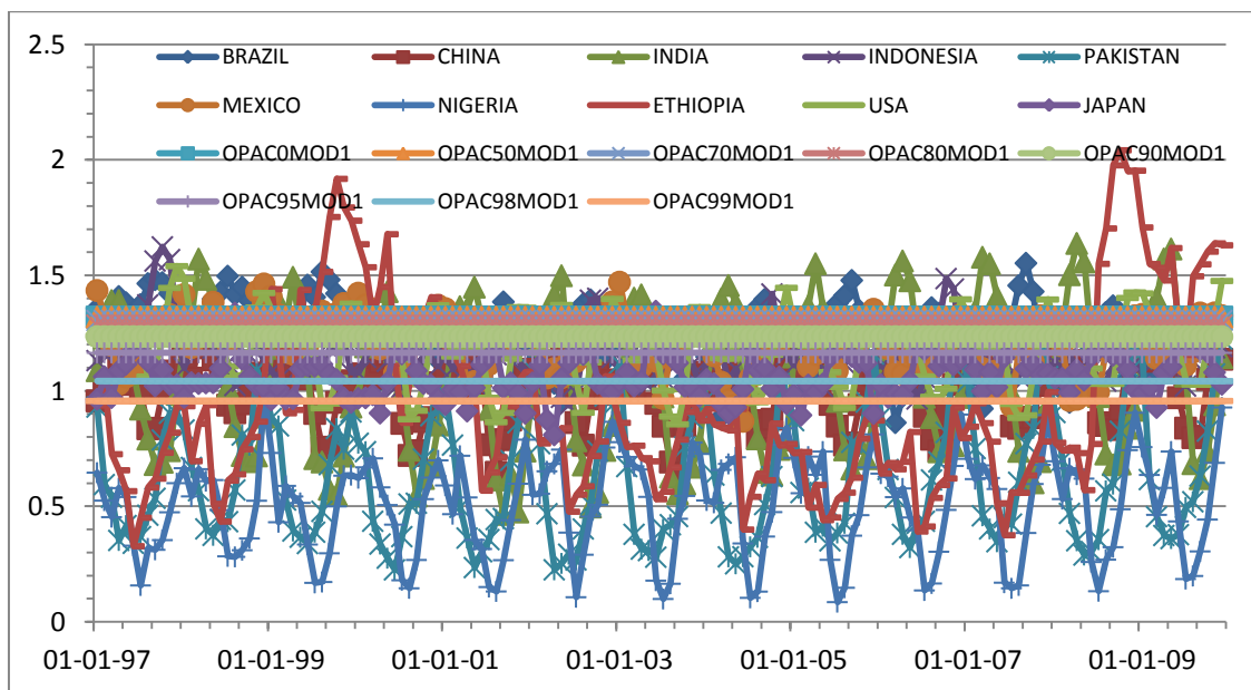
Fig. 6. Angstrom Exponent ( \alpha ) plot for OPAC INSO Model 1 Angstrom Exponent ( \alpha ) and MERRA averaged Angstrom Exponent ( \alpha ) for ten countries (Nigeria, Ethiopia, Brazil, USA, Pakistan, Mexico, Japan, China, Indonesia and India)
