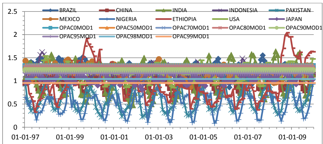
Fig. 2. Angstrom Exponent ( \alpha ) plot for OPAC WASO Model 1 Angstrom Exponent ( \alpha ) and MERRA averaged Angstrom Exponent ( \alpha ) for ten countries
