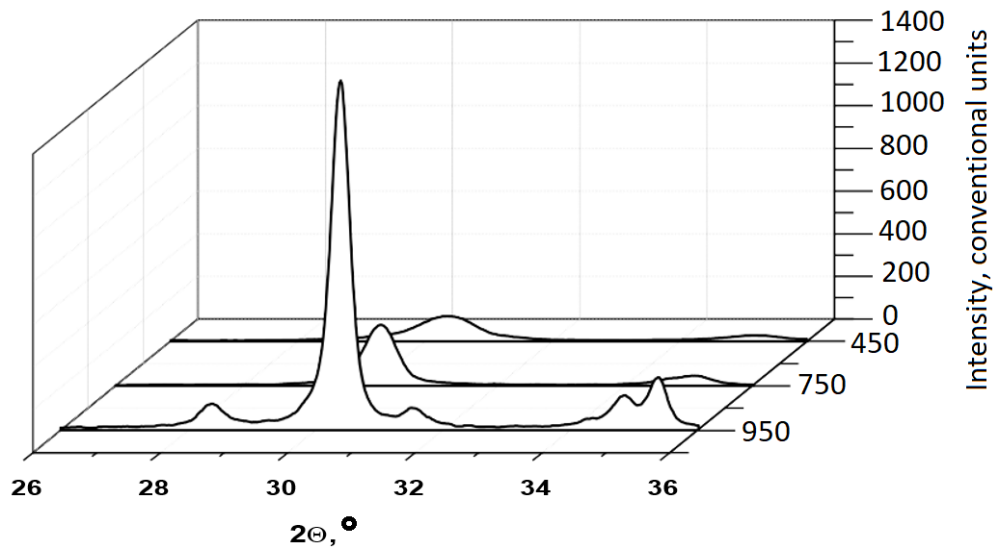
Fig. 1. Fragments of diffractograms of Yb–TZP powders
