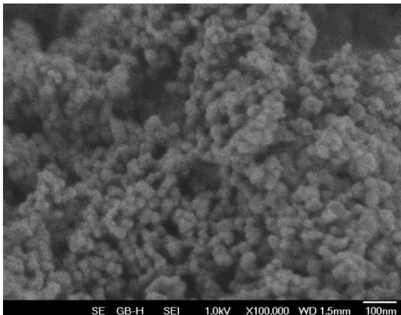
Fig. 2. Electronic micrography of powder
