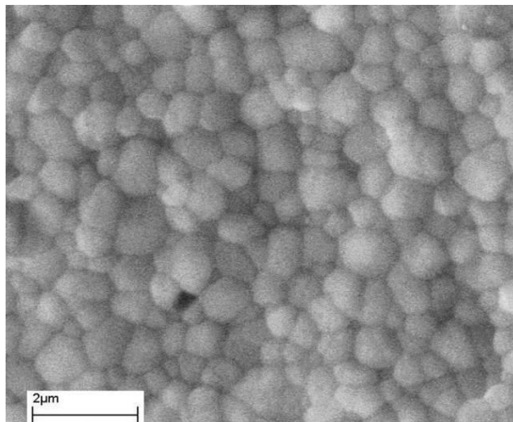
Fig. 3. Microstructure of sintered ceramics Yb-TZP
