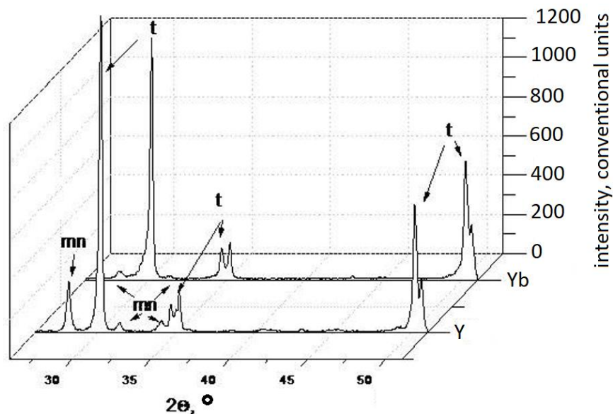
Fig. 4. Fragments of diffractograms of the surface of Y-TZP and Yb-TZP samples after exposure to hydrothermal treatment
