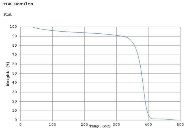
Fig. 7. Graph of weight loss % versus temperature
