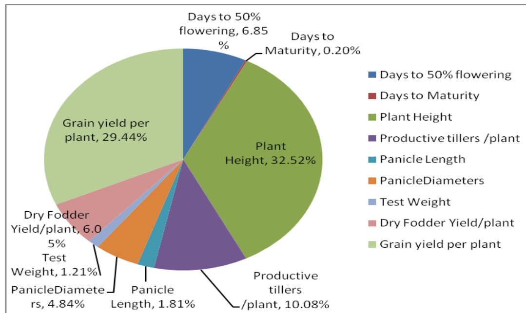
Fig. 2. % contribution of 12 biometrical traits towards genetic divergence
