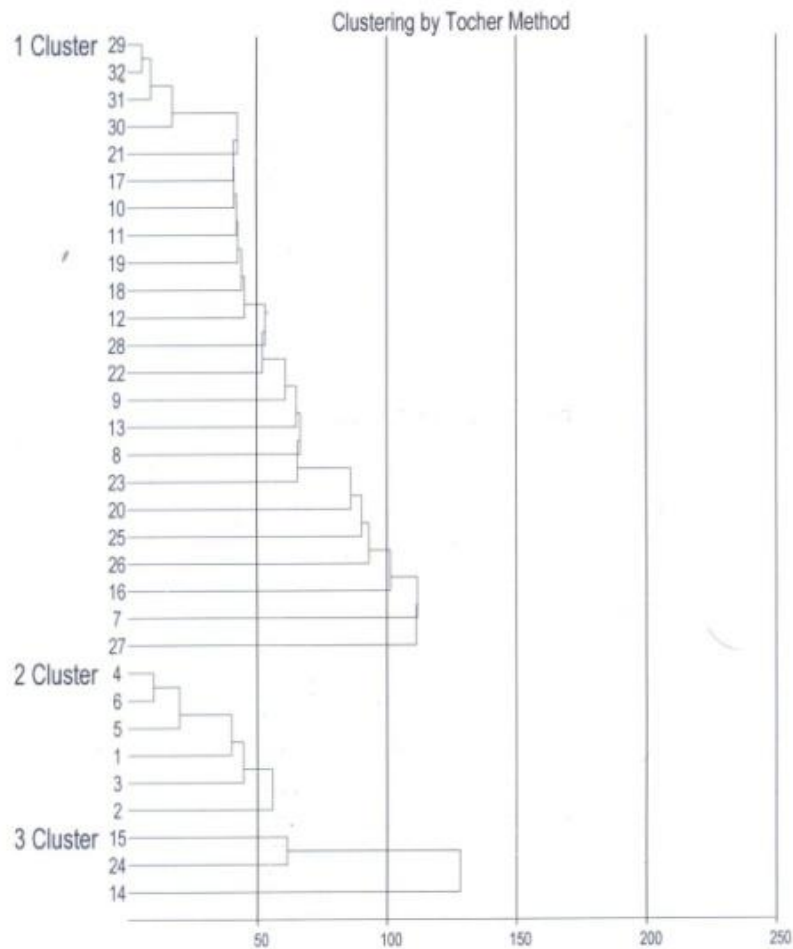
Fig. 1. Dendrogram for 9 biometrical traits towards genetic divergence
